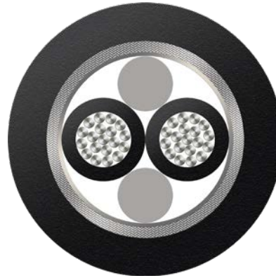
SeaLine® BWTS Cable 1x2x0.75 VZN BK Order no.: L45551-D21-K16
