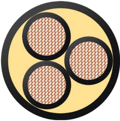
SeaLine® BWTS Cable 3x1x35.0 BK Order no.: L45550-D31-K6
