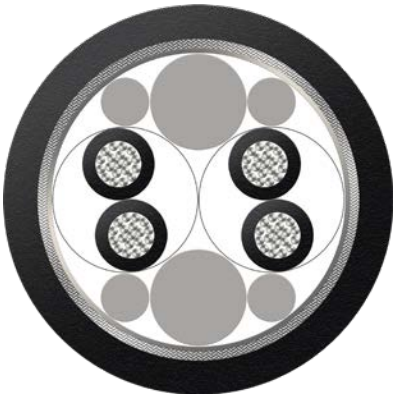
SeaLine® BWTS Cable 2x2x0.75 VZN BK Order no.: L45551-D22-K16
